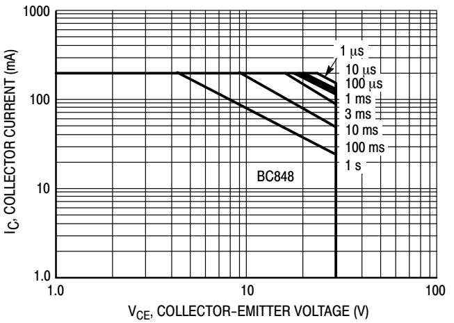
Figure 52. Safe Operating Area – BC848
