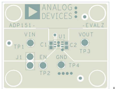
Figure 62. Example LFCSP PCB Layout
