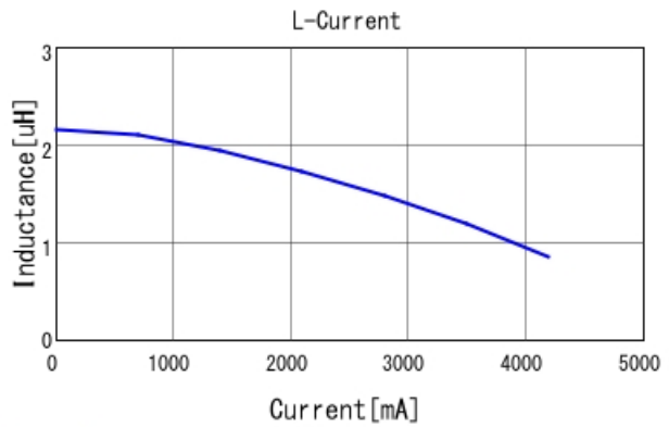
DFE201612E-2R2M L-Current 20degC
