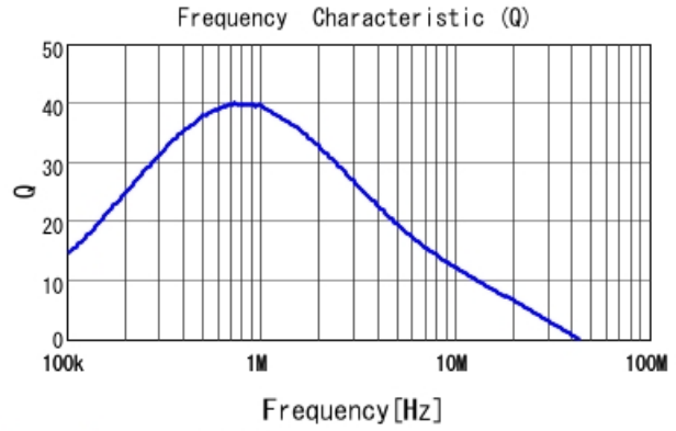
DFE201612E-2R2M Q
