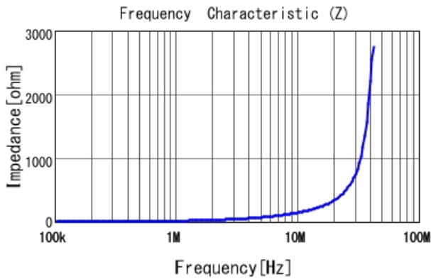
DFE201612E-2R2M |Z|
