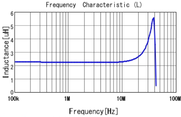
DFE201612E-2R2M L
