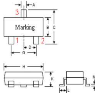
SOT-323: 1: Base 2: Emitter 3: Collector
