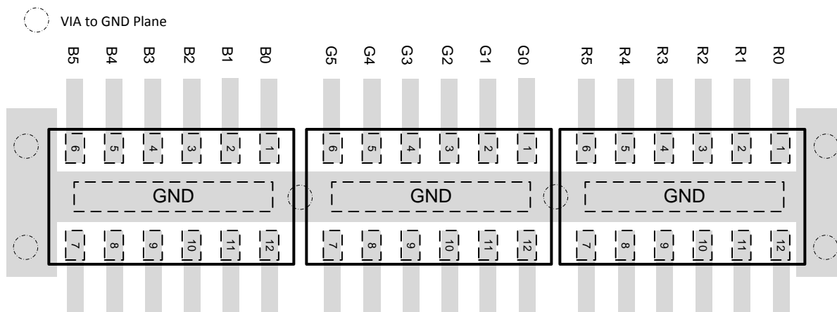
Figure 12. TPD6F003 Layout
