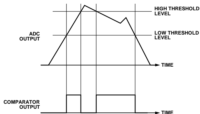
Figure 29. Comparator Behavior in Midrange Output Mode
