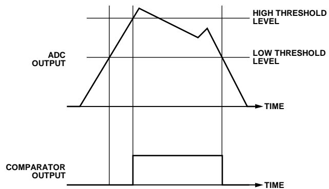
Figure 28. Comparator Behavior in Hysteretic Output Mode
