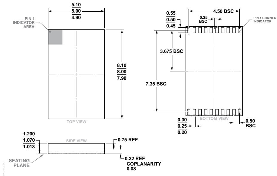
Figure 53. 20-Lead Land Grid Array [LGA] (CC-20-5) Dimensions shown in millimeters
