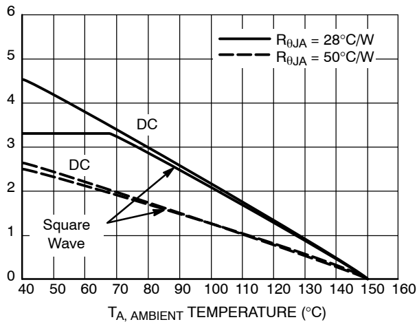
Figure 4. Maximum Current Derating, Ambient, PC Board Mounting
