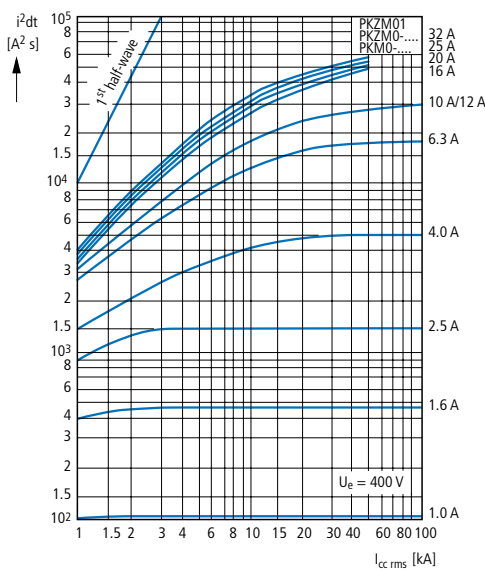
Let-through characteristics, motor-protective circuit breaker, transformer-protective circuit breaker, circuit breaker for starter combinations
