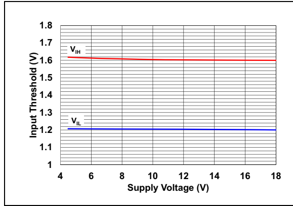
FIGURE 2-16: Input Threshold vs. Supply Voltage.
