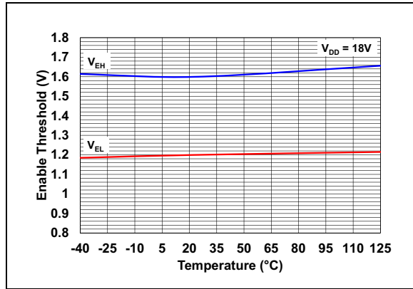
FIGURE 2-17: Enable Threshold vs. Temperature.
