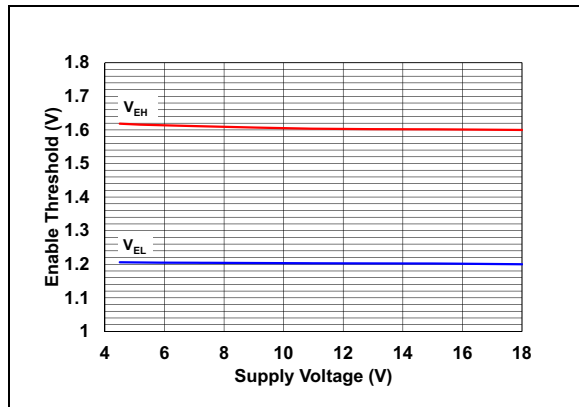
FIGURE 2-18: Enable Threshold vs. Supply Voltage.
