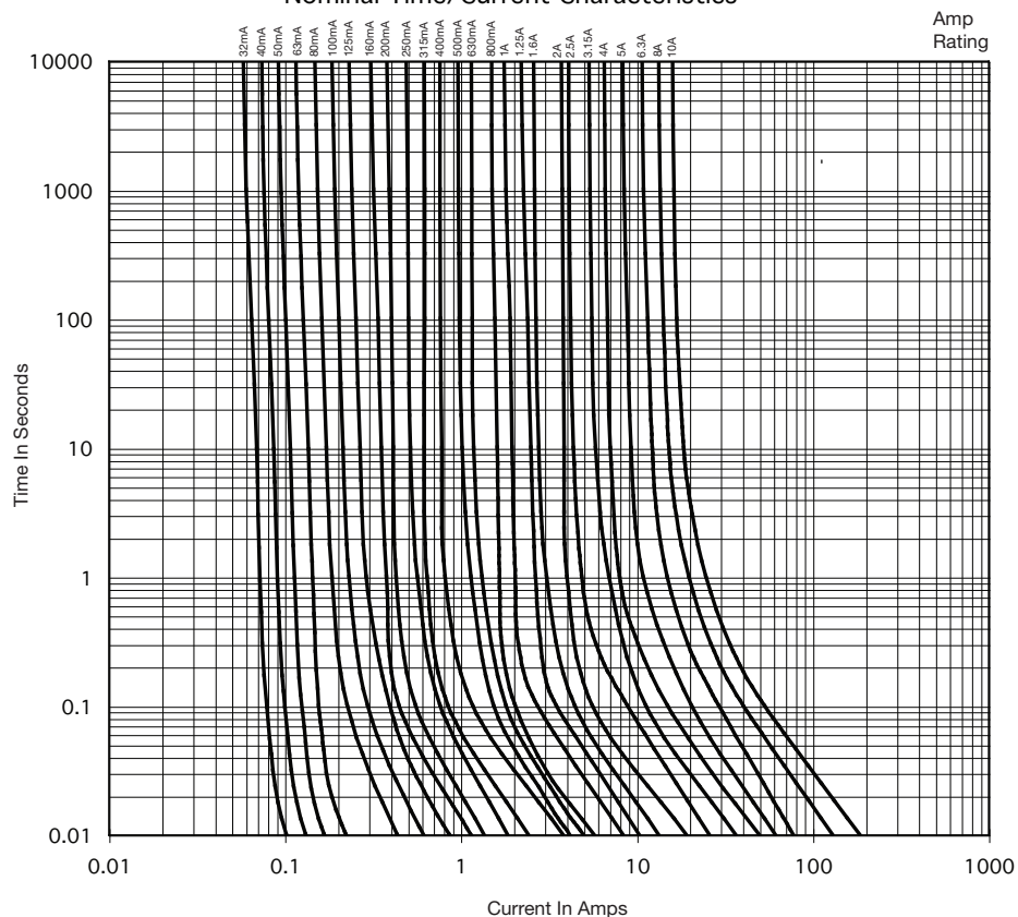
Time-current Curve Nominal Time/Current Characteristics
