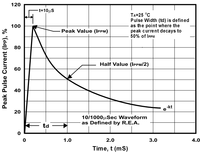
FIGURE 3. PULSE WAVEFORM
