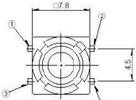
Outline Drawing
