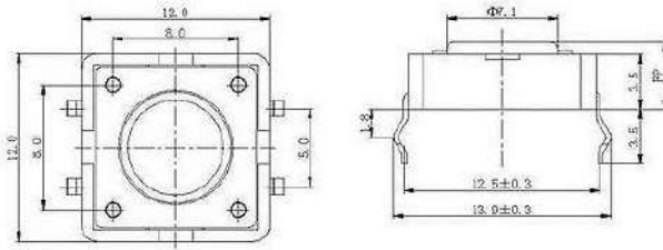
Outline Drawing
