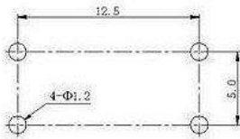
Mounting
