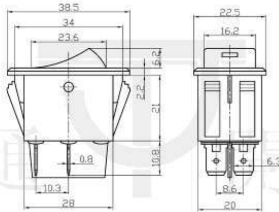
Outline Drawing
