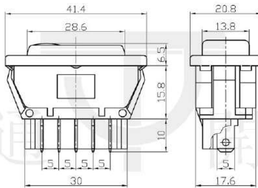
Mounting
