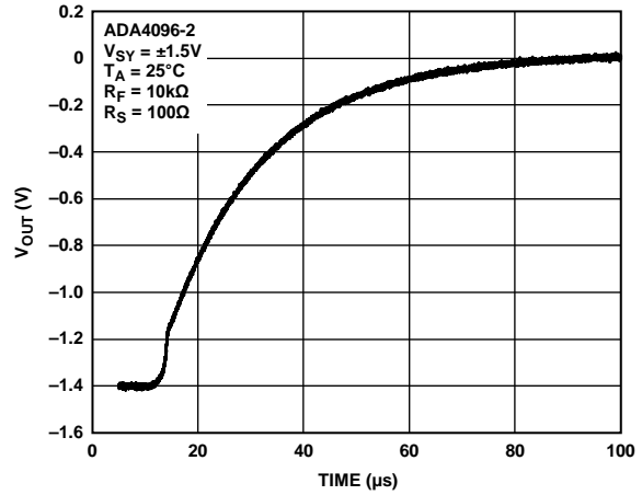
Figure 20. Negative Overload Recovery
