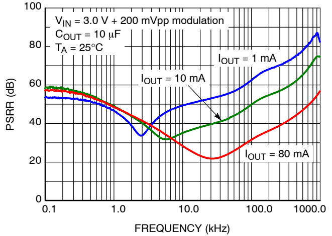
Figure 22. NCV8716x15xxx PSRR vs. Frequency
