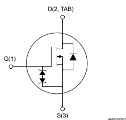
TO-247 long leads
