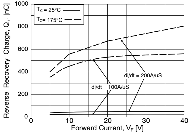
Figure 18. Stored Charge
