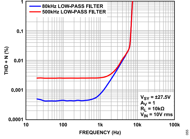
Figure 53. THD + N vs. Frequency, V_{SY} = \pm 27.5\text{ V}
