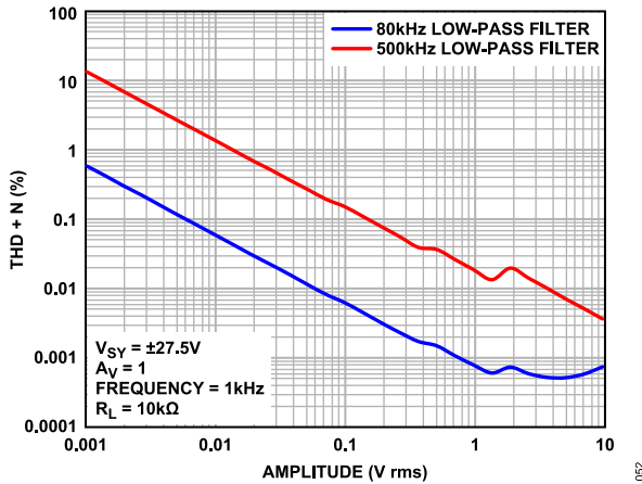
Figure 50. THD + N vs. Amplitude, V_{SY} = \pm 27.5\text{ V}
