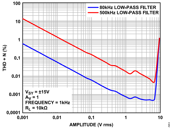
Figure 49. THD + N vs. Amplitude, V_{SY} = \pm 15\text{ V}
