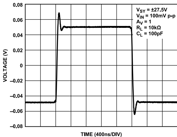
Figure 41. Small Signal Transient Response, V_{SY} = \pm 27.5\text{ V}
