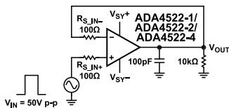
Figure 75. Circuit Diagram for Large Signal Transient Response
