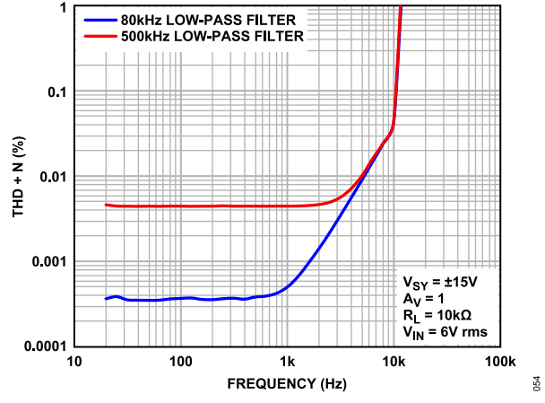
Figure 52. THD + N vs. Frequency, V_{SY} = \pm 15\text{ V}
