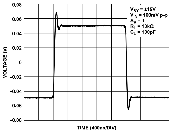
Figure 40. Small Signal Transient Response, V_{SY} = \pm 15\text{ V}
