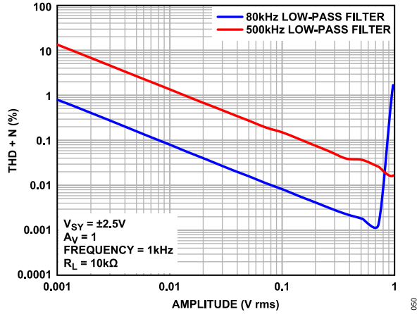
Figure 48. THD + N vs. Amplitude, V_{SY} = \pm 2.5\text{ V}
