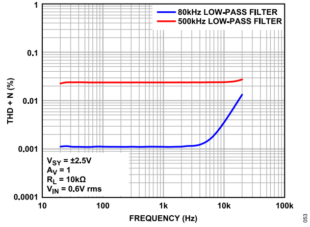
Figure 51. THD + N vs. Frequency, V_{SY} = \pm 2.5\text{ V}
