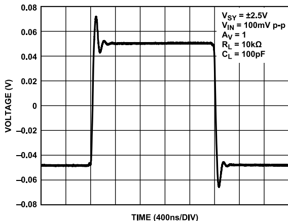
Figure 39. Small Signal Transient Response, V_{SY} = \pm 2.5\text{ V}
