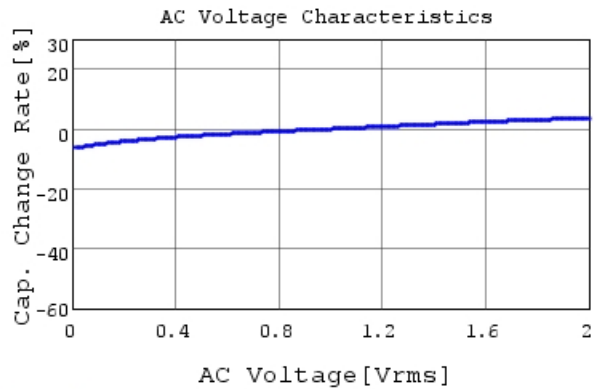
GRT155R71C104KE01 C-AC Voltage capchange, Dc
