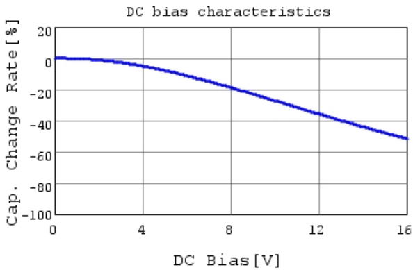
GRT155R71C104KE01 C-DC bias capchange, 25.0c
