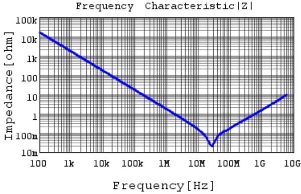
GRT155R71C104KE01 |Z| DCOV, 25degC
