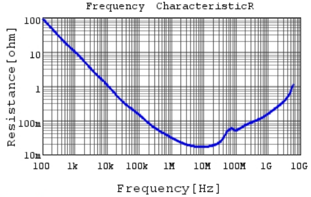
GRT155R71C104KE01 R DCOV, 25degC
