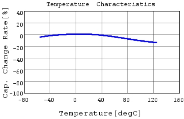
GRT155R71C104KE01 C-Temp. capchange, DC0.0V,
