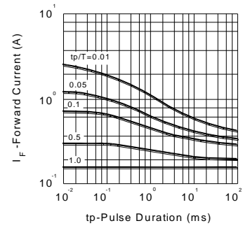
FIG.7 PULSE FORWARD CURRENT VS. PULSE DURATION
