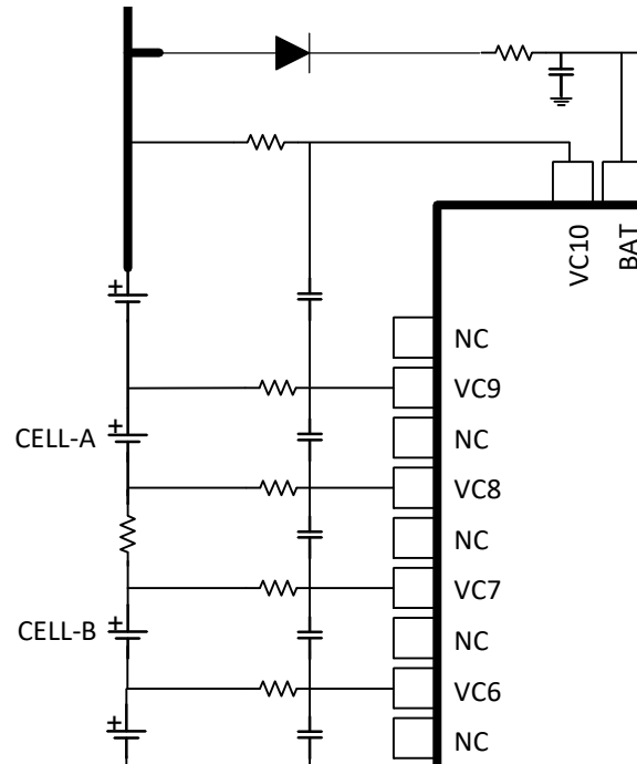
Figure 10-1. Using Cell Input Pins for Interconnect Measurement
