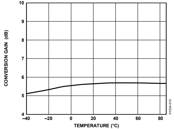
Figure 10. Gain Performance Over Temperature; f_{IN} = 400\text{ MHz} , f_{OUT} = 70\text{ MHz}
