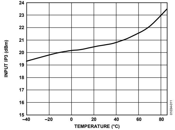
Figure 11. Input IP3 Performance Over Temperature; f_{IN} = 400\text{ MHz} , f_{OUT} = 70\text{ MHz}
