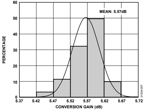
Figure 7. Gain Histogram; f_{IN} = 400\text{ MHz} , f_{OUT} = 70\text{ MHz}
