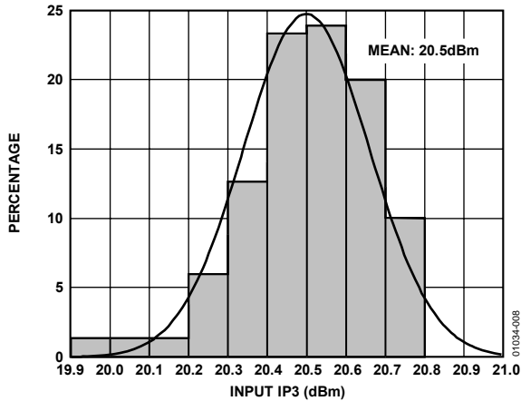
Figure 8. Input IP3 Histogram; f_{IN} = 400\text{ MHz} , f_{OUT} = 70\text{ MHz}
