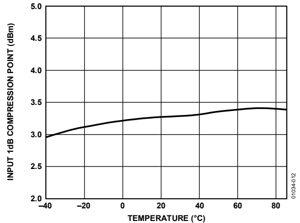
Figure 12. Input 1 dB Compression Point Performance Over Temperature; f_{IN} = 400\text{ MHz} , f_{OUT} = 70\text{ MHz}
