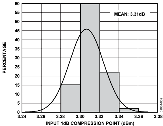
Figure 9. Input 1 dB Compression Point Histogram; f_{IN} = 400\text{ MHz} , f_{OUT} = 70\text{ MHz}
