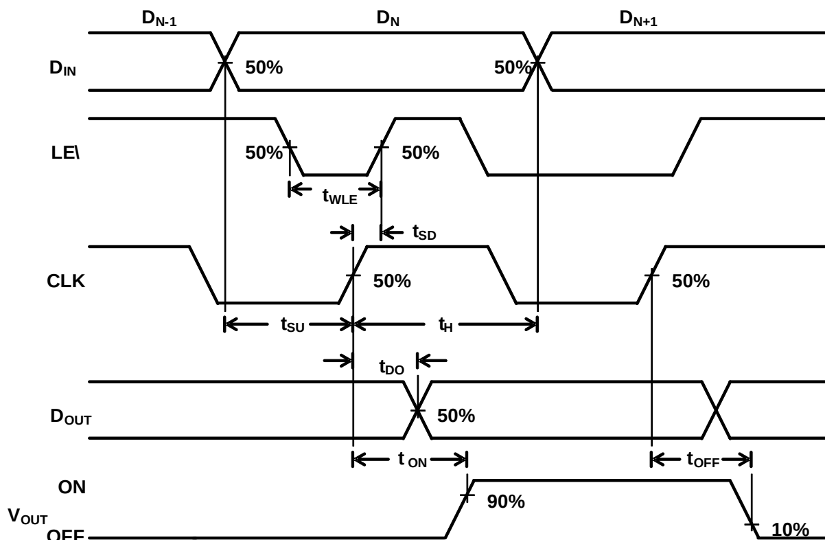
Figure 1: Timing Diagram
