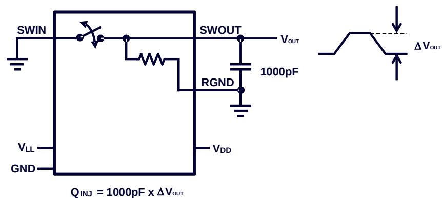
Figure 8: Test Circuit 7
