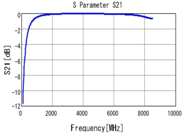
■ GRM1555C1H4R3WA01 S21 DCOV, 25degC
