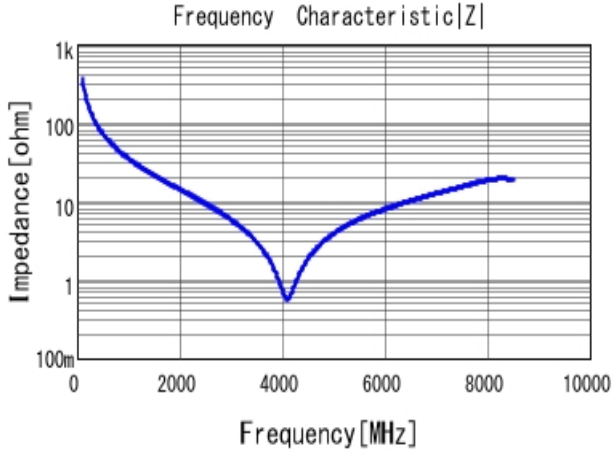
■ GRM1555C1H4R3WA01 |Z| DC0V, 25degC
