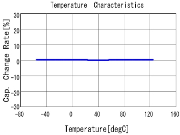
■ GRM1555C1H4R3WA01 C-Temp. capchange, DCOV, AC1Vrms
