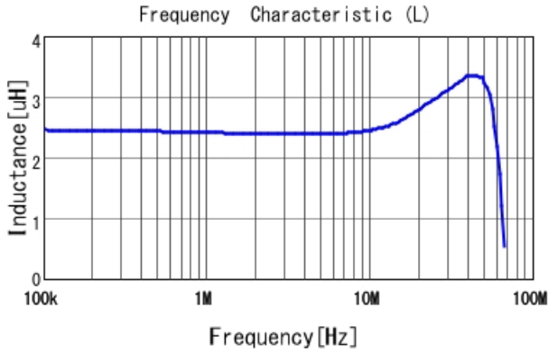
■ LQM2MPN2R2MG0 L
