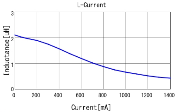
■ LQM2MPN2R2MG0 L-Current 20degC
