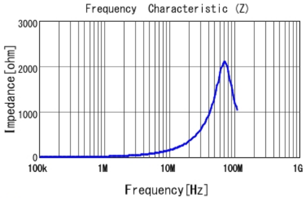
■ LQM2MPN2R2MG0 |Z|
