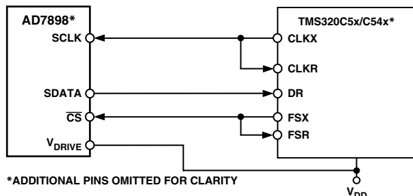
Figure 17. AD7898 to TMS320C5x Interface
