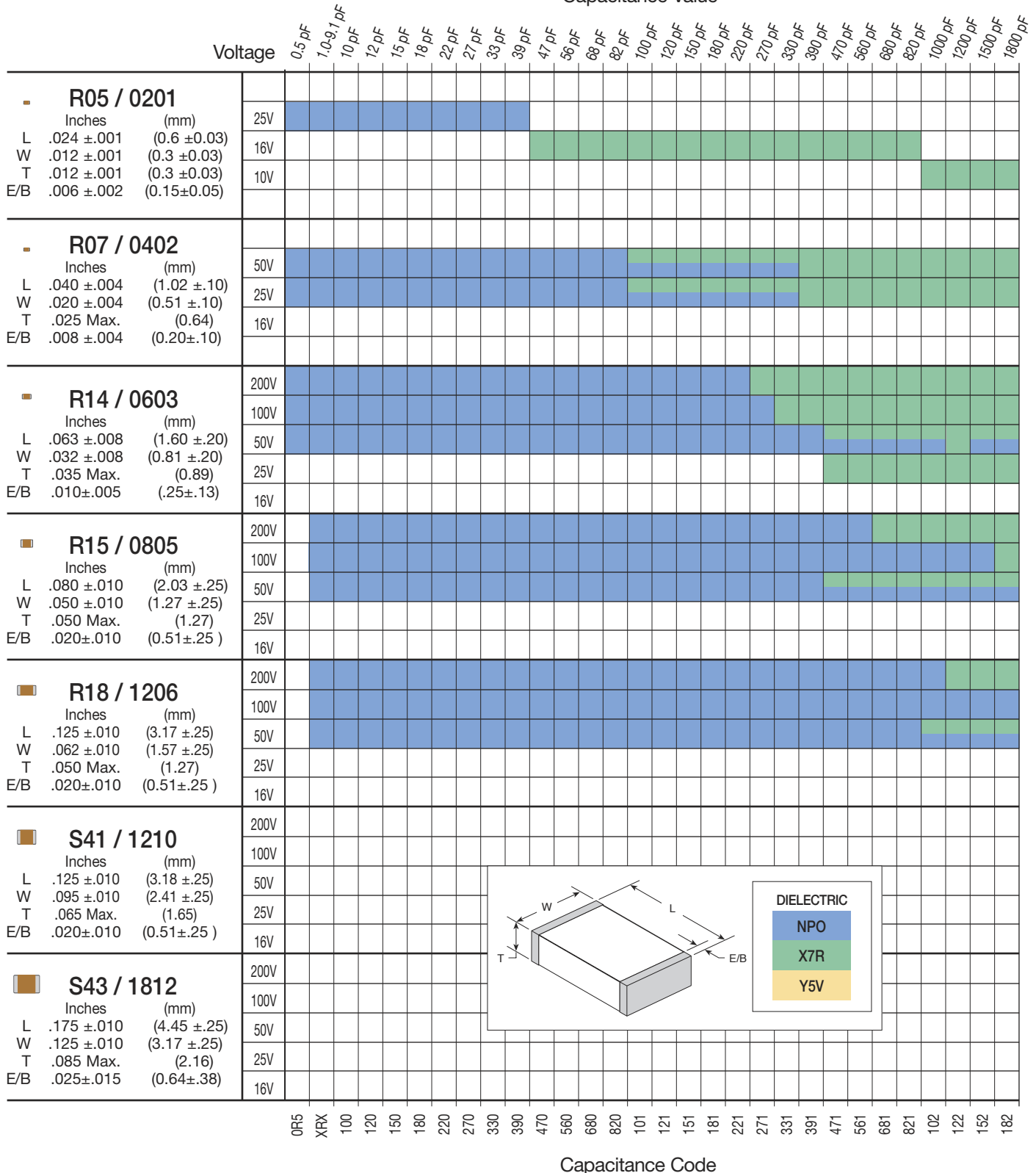
Capacitance Value
