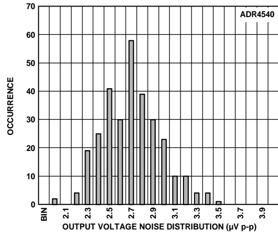
Figure 74. ADR4540 Output Voltage Noise (Maximum Amplitude from 0.1 Hz to 10 Hz)
