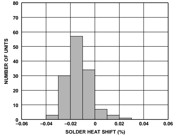
Figure 64. ADR4533 Solder Heat Resistance Shift (3 × Reflow)
