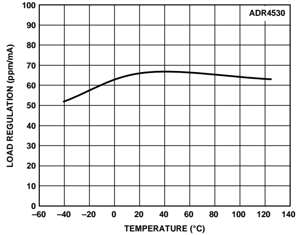
Figure 43. ADR4530 Load Regulation vs. Temperature (Sinking)
