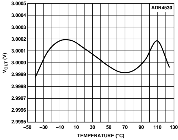
Figure 39. ADR4530 B Grade Output Voltage vs. Temperature
