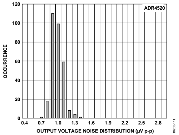
Figure 12. ADR4520 Output Voltage Noise (Maximum Amplitude from 0.1 Hz to 10 Hz)
