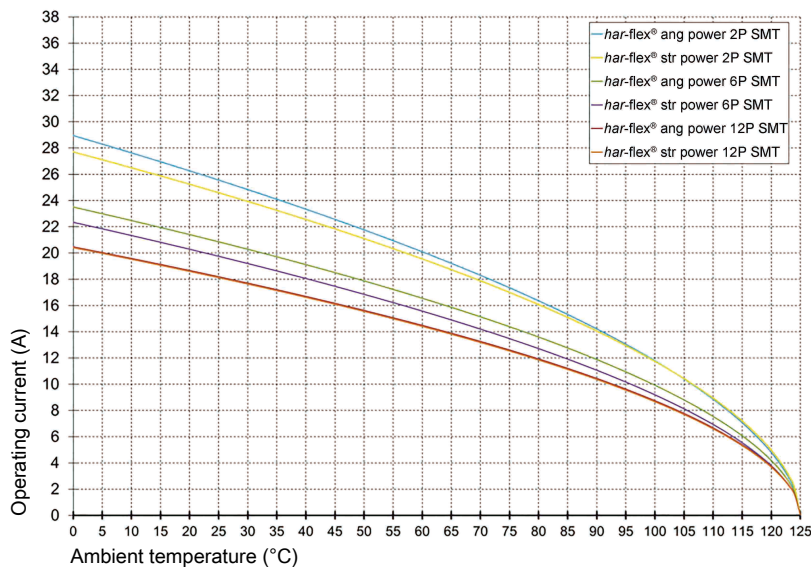
Derating curve 80%
