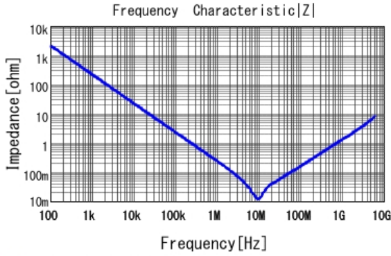
■ GRM155R6YA105KE11 |Z| DCOV, 25degC
