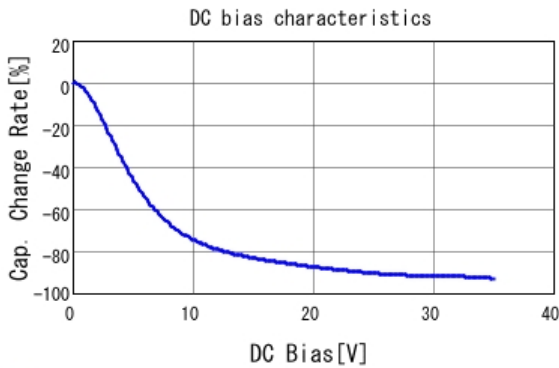
■ GRM155R6YA105KE11 C-DC bias capchange, 25.0degC, AC1V
