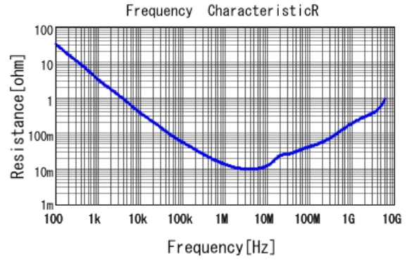
■ GRM155R6YA105KE11 R DCOV, 25degC
