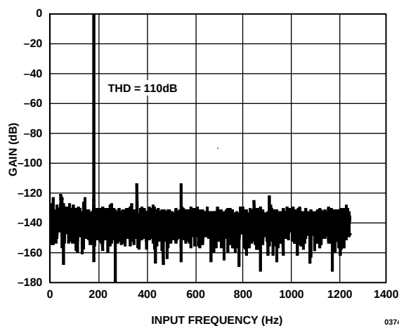
Figure 8. Typical FFT Plot; Input Sine Wave 183 Hz, 1.2 V Peak, AIN Range \pm 1.25 V, Conversion Time 397 \mu s, Chopping Enabled, MCLK = 6.144 MHz
