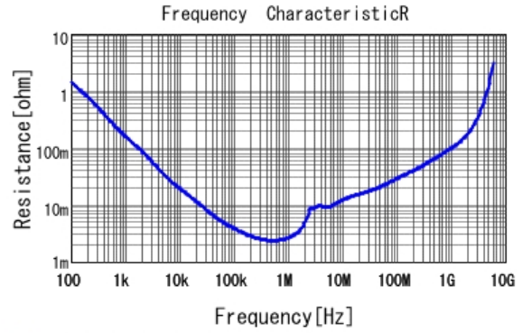
■ GRM21BC81C226ME44 R DCOV, 25degC
