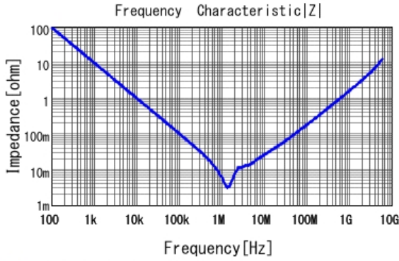
■ GRM21BC81C226ME44 |Z| DCOV, 25degC
