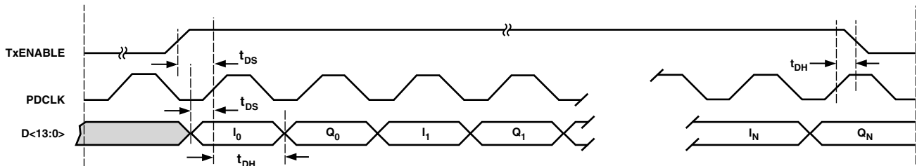
Figure 4. 14-Bit Parallel Port Timing Diagram—Quadrature Modulation Mode
