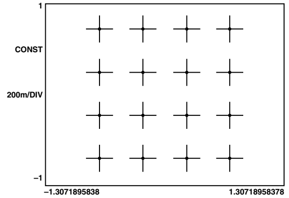
TPC 14. 16-QAM, 65 MHz, 2.56 MS/s
