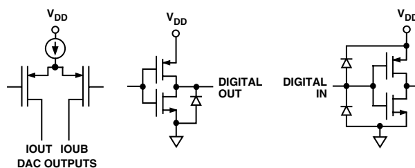
Figure 18. Equivalent I/O Circuits
