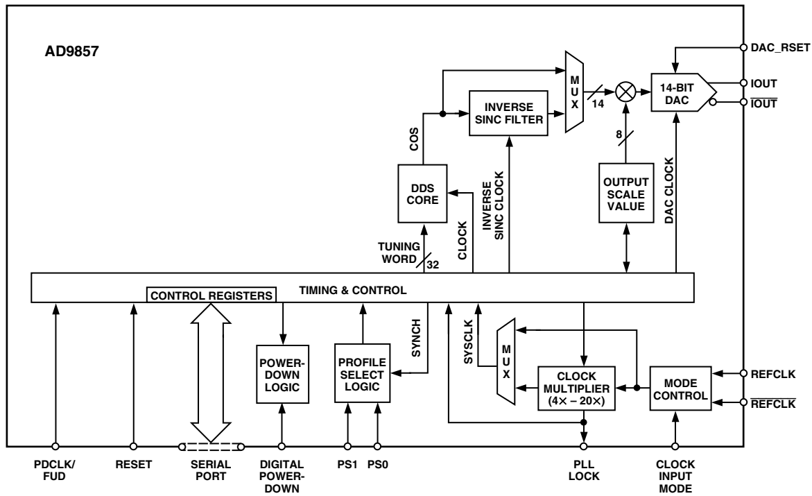
Figure 2. Single-Tone Mode
