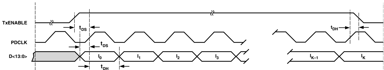
Figure 5. 14-Bit Parallel Port Timing Diagram—Interpolating DAC Mode
