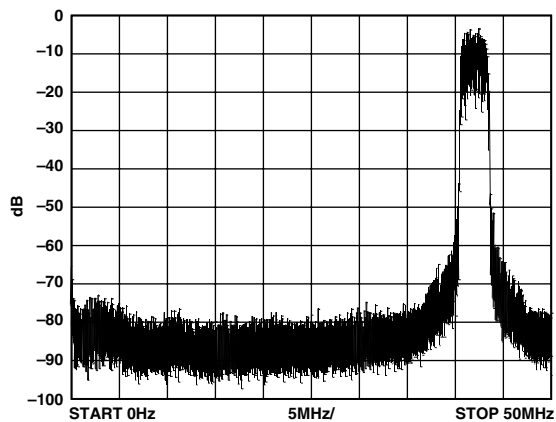
TPC 1. QPSK at 42 MHz and 2.56 MS/s; 10.24 MHz External Clock with REFCLK Multiplier = 12, CIC Interpolation Rate = 3, 4× Oversampled Data
