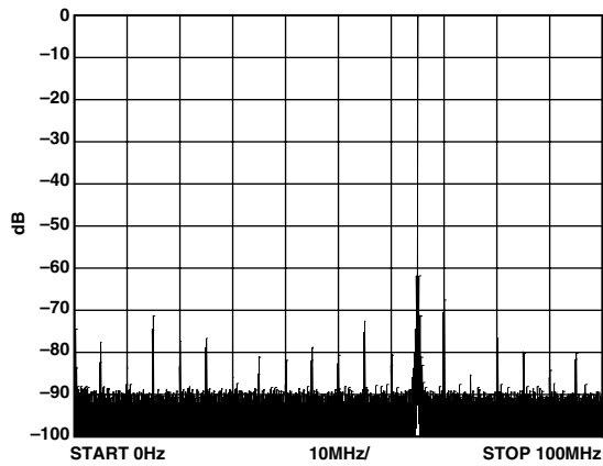
TPC 6. 65 MHz Single-Tone Output
