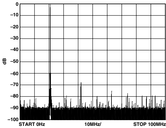
TPC 5. 21 MHz Single-Tone Output
