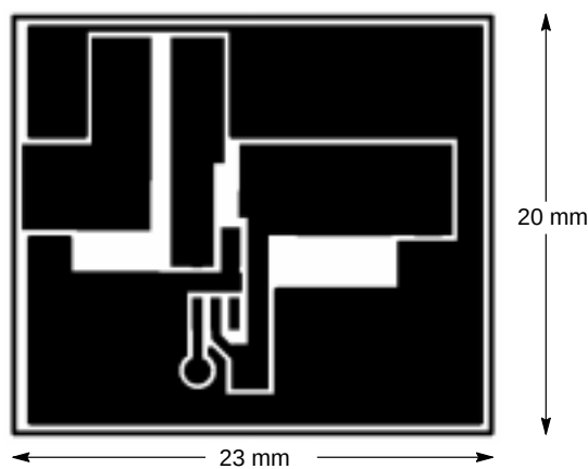
Figure 43. NCP1400A PWM Step-up DC-DC Converter Evaluation Board Artwork (Component Side)
