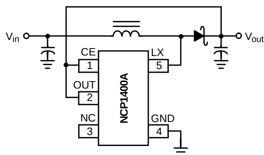
Figure 1. Typical Step-Up Converter Application
