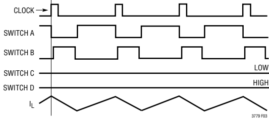
Figure 3. Buck Region ( V_{IN} \gg V_{OUT} )
