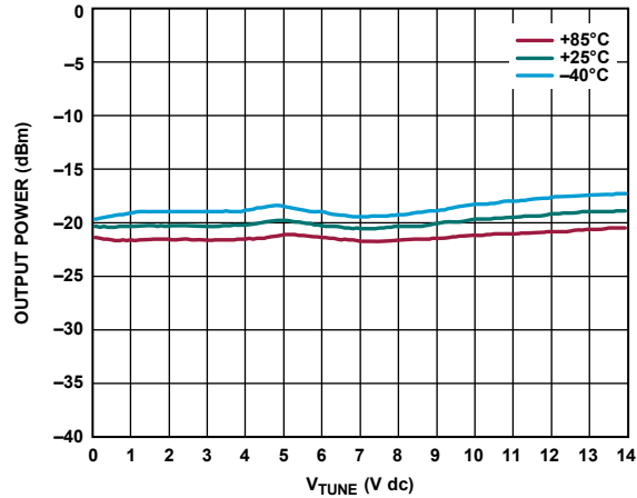
Figure 26. Output Power vs. V_{TUNE} at V_{CB} = 0 V for Various Temperatures
