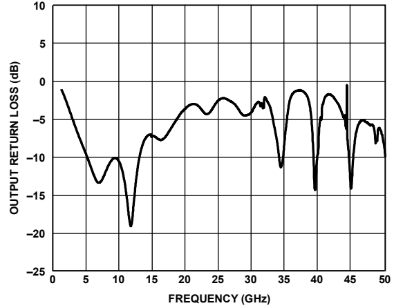
Figure 25. Output Return Loss vs. Frequency at V_{TUNE} = 7.25 V, V_{CB} = 5 V, T_A = 25^\circ\text{C}
