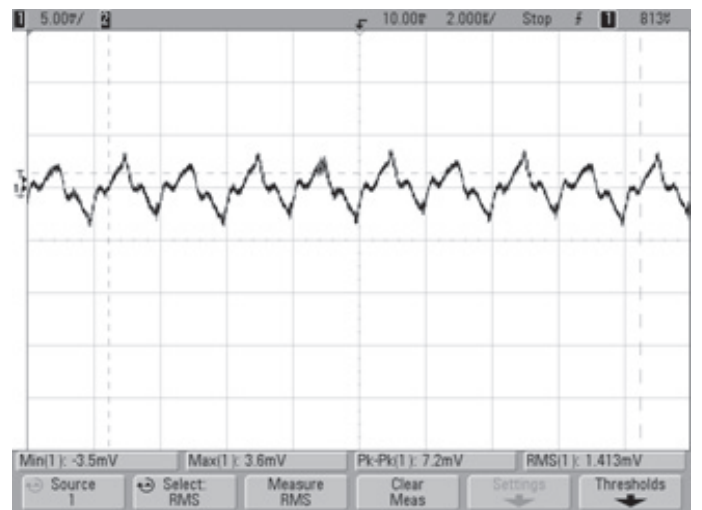
Output Ripple and noise (VIN = 48V, Vout = nom, Iout = 0A, Load = 330uF, Ta = +25°C)
