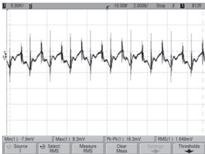
Output Ripple and noise (VIN = 48V, Vout = nom, Iout = 20A, Load = 330uF, Ta = +25°C)
