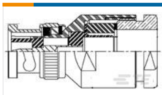
TE Part #1-1337447-0 BNC Ins BHSkt 50Ohm Nickel Silver Pltd
