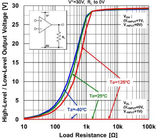
High-Level / Low-Level Output Voltage vs. Load Resistance V^+ = 30V, R_L to 0V
