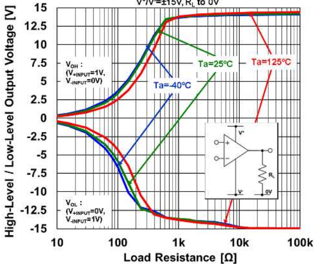
High-Level / Low-Level Output Voltage vs. Load Resistance V^+ = 30V, R_L to 0V
