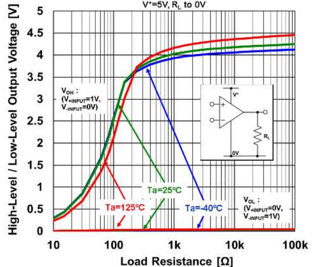
High-Level / Low-Level Output Voltage vs. Load Resistance V^+ = 5V, R_L to 0V
