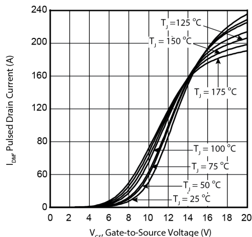
Figure 8 • I_{DM} vs. V_{GS}
