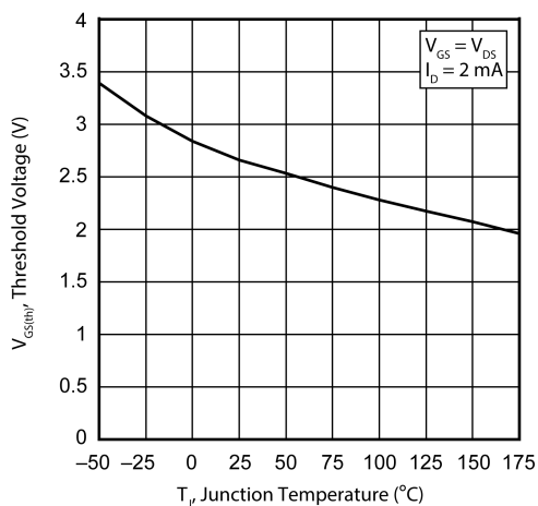
Figure 11 • V_{GS(th)} vs. Junction Temperature
