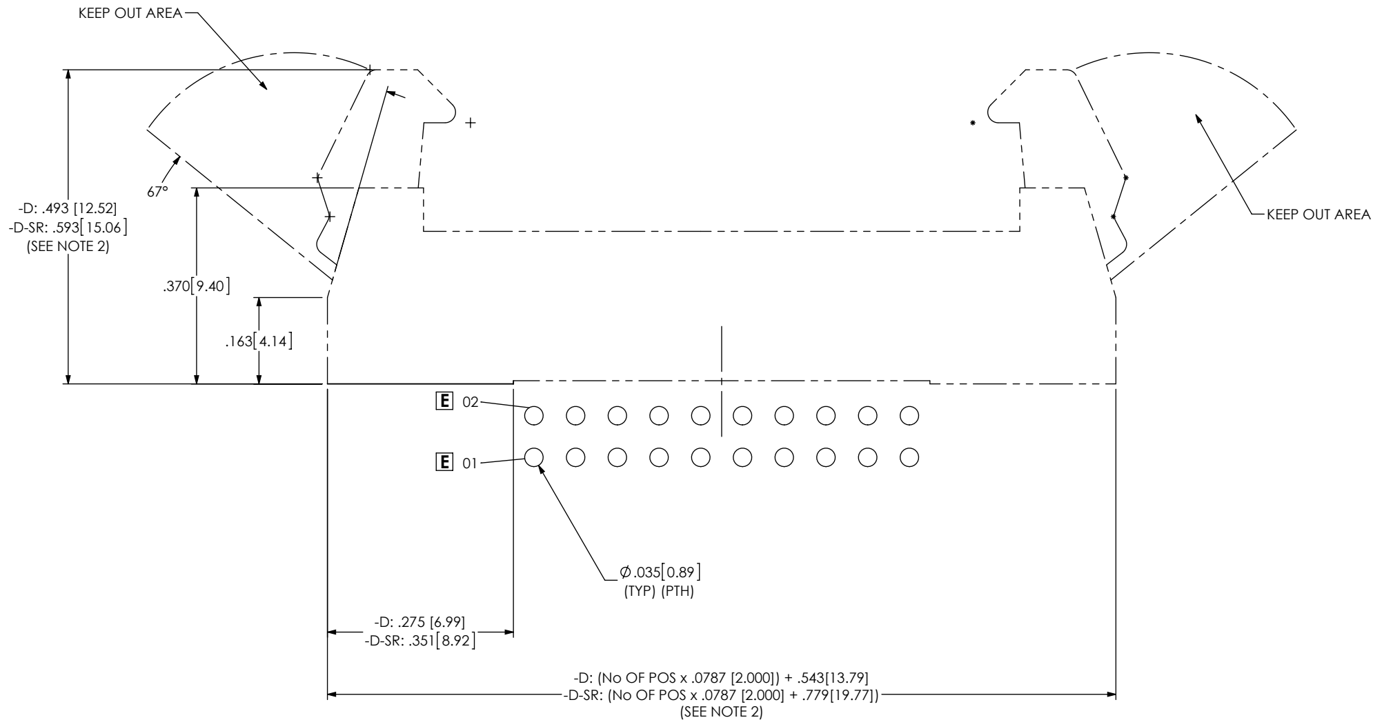
FIG 5 EHT-110-01-X-D-RA & EHT-110-01-X-D-RA-SR SHOWN (DIFFERENT AS SHOWN, OTHERWISE SAME AS FIG 4)
