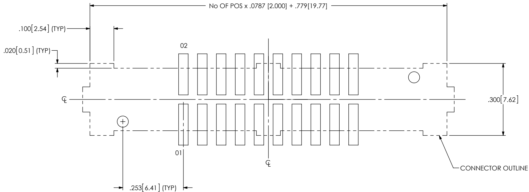
FIG 2 EHT-110-01-X-D-SM-SR-LC SHOWN (DIFFERENT AS SHOWN, OTHERWISE SAME AS FIG 1)
