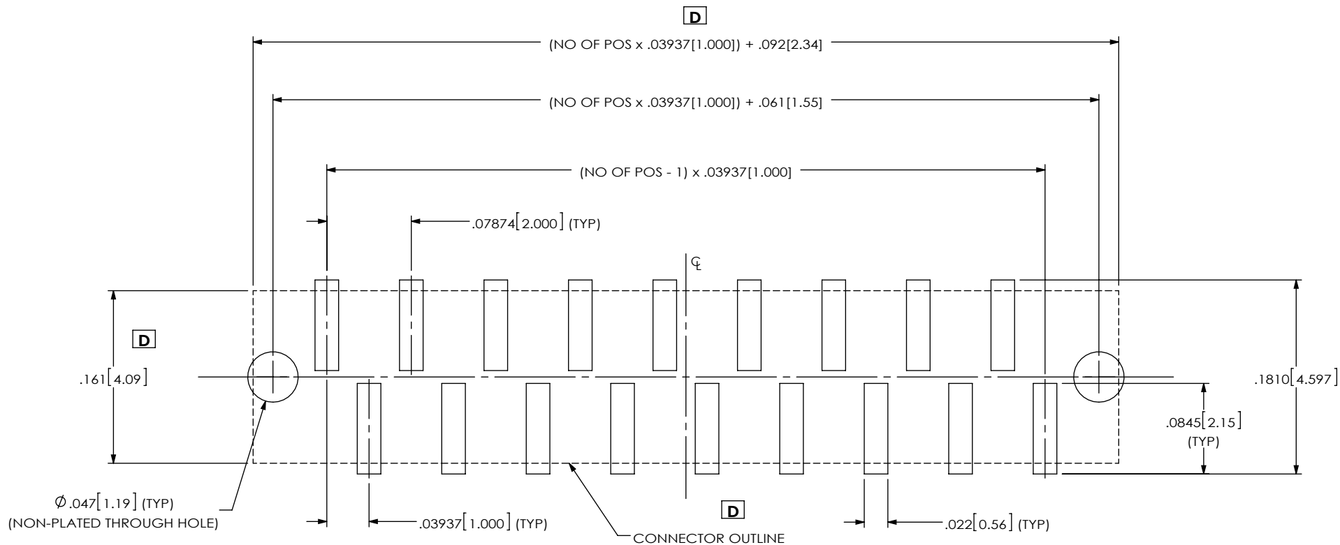
FIG 1 FOOTPRINT FOR FC1-XX-X1-XX-LC SHOWN
