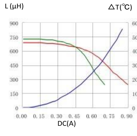
18. CDRH125L125NP-681MC
