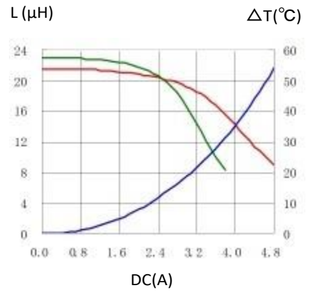
9. CDRH125L125NP-220MC
