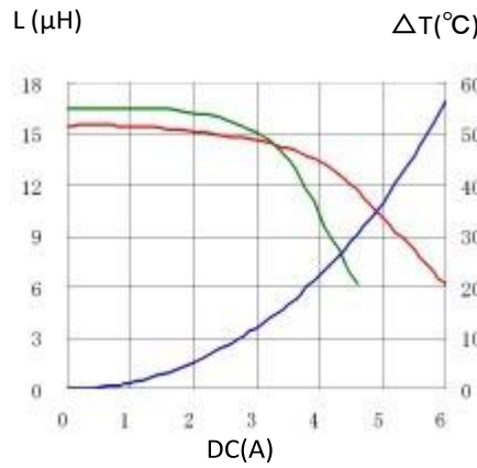
8. CDRH125L125NP-150MC
