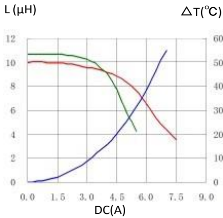
7. CDRH125L125NP-100MC
