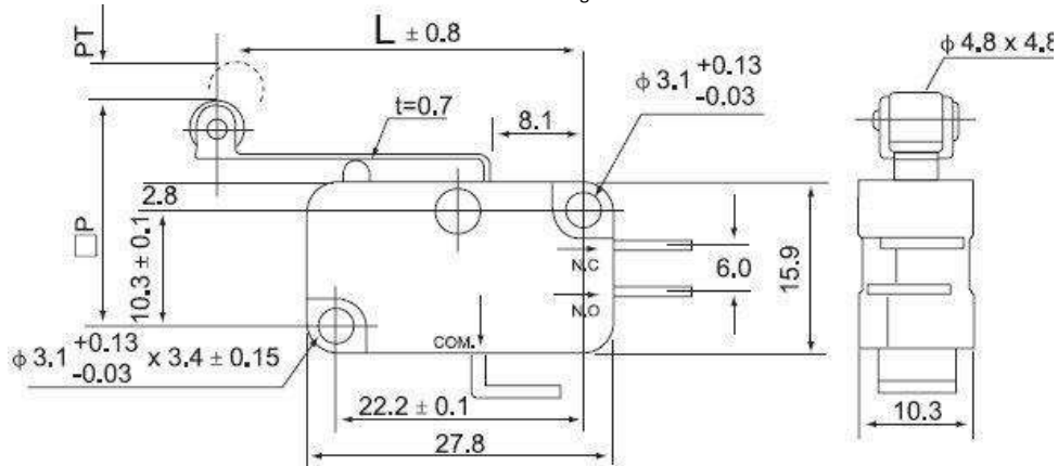
Outline Drawing
