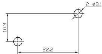
Mounting
