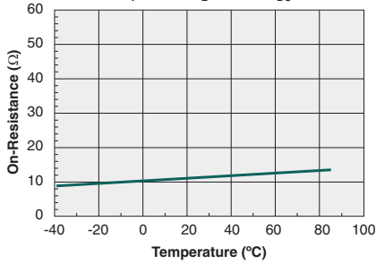
Form-B Typical On-Resistance vs. Temperature ( I_F=0\text{mA} , I_L=170\text{mA}_{DC} )
