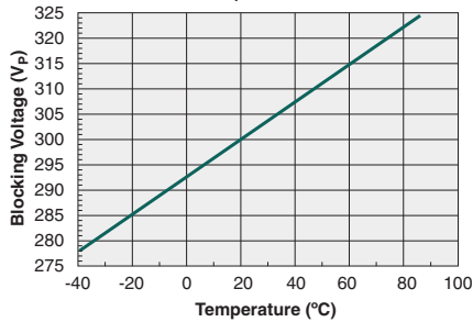
Form-B Typical Blocking Voltage vs. Temperature ( I_F=5\text{mA} )
