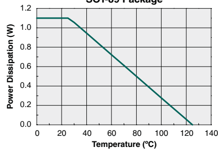
Power Dissipation vs. Ambient Temperature SOT-89 Package
