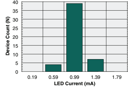
Typical I F for Switch Dropout (N=50, I F =5mA, I L =100mA DC )
