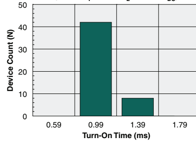
Typical Turn-On Time Distribution (N=50, I F =5mA, I L =100mA DC )
