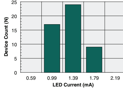
Typical I F for Switch Operation (N=50, I F =5mA, I L =100mA DC )
