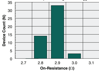
Typical On-Resistance Distribution (N=50, I F =5mA, I L =100mA DC )
