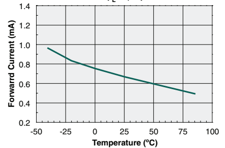
Typical I F for Switch Dropout vs. Temperature (I L =1μA)
