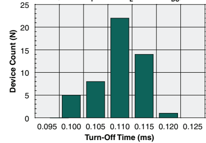
Typical Turn-Off Time Distribution (N=50, I F =5mA, I L =100mA DC )
