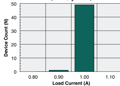
Typical Current Limit Distribution (N=50, I F =5mA)
