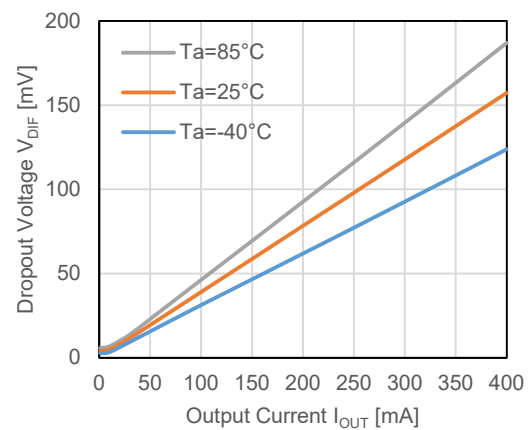
RP122K/N281x
