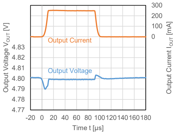
RP122x48xx, V_{IN} = 5.5\text{ V} , I_{OUT} = 1\text{ mA} \Leftrightarrow 250\text{ mA} , t_R = t_F = 10\ \mu\text{s}
